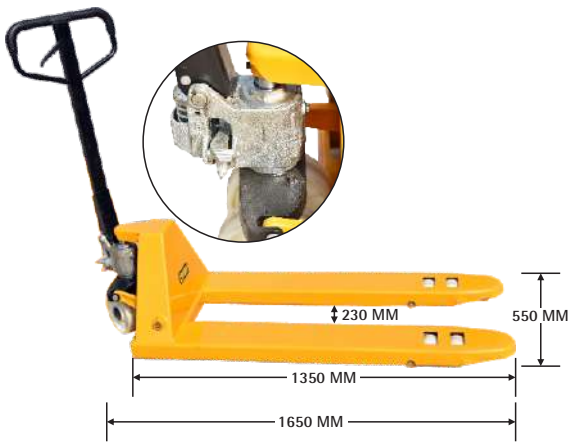
Hydraulic Hand Pallet Truck Cap.: 2, 2.5, 3 Ton Size : 1150 x 550, 1220 x 685 (mm)
